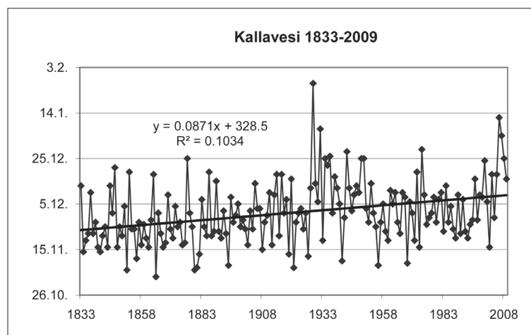
Figure 1: Freezing dates of Lake Kallavesi 1833–2009.
