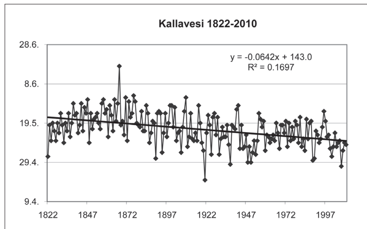
Figure 2: Break-up dates of Lake Kallavesi 1822–2010.
